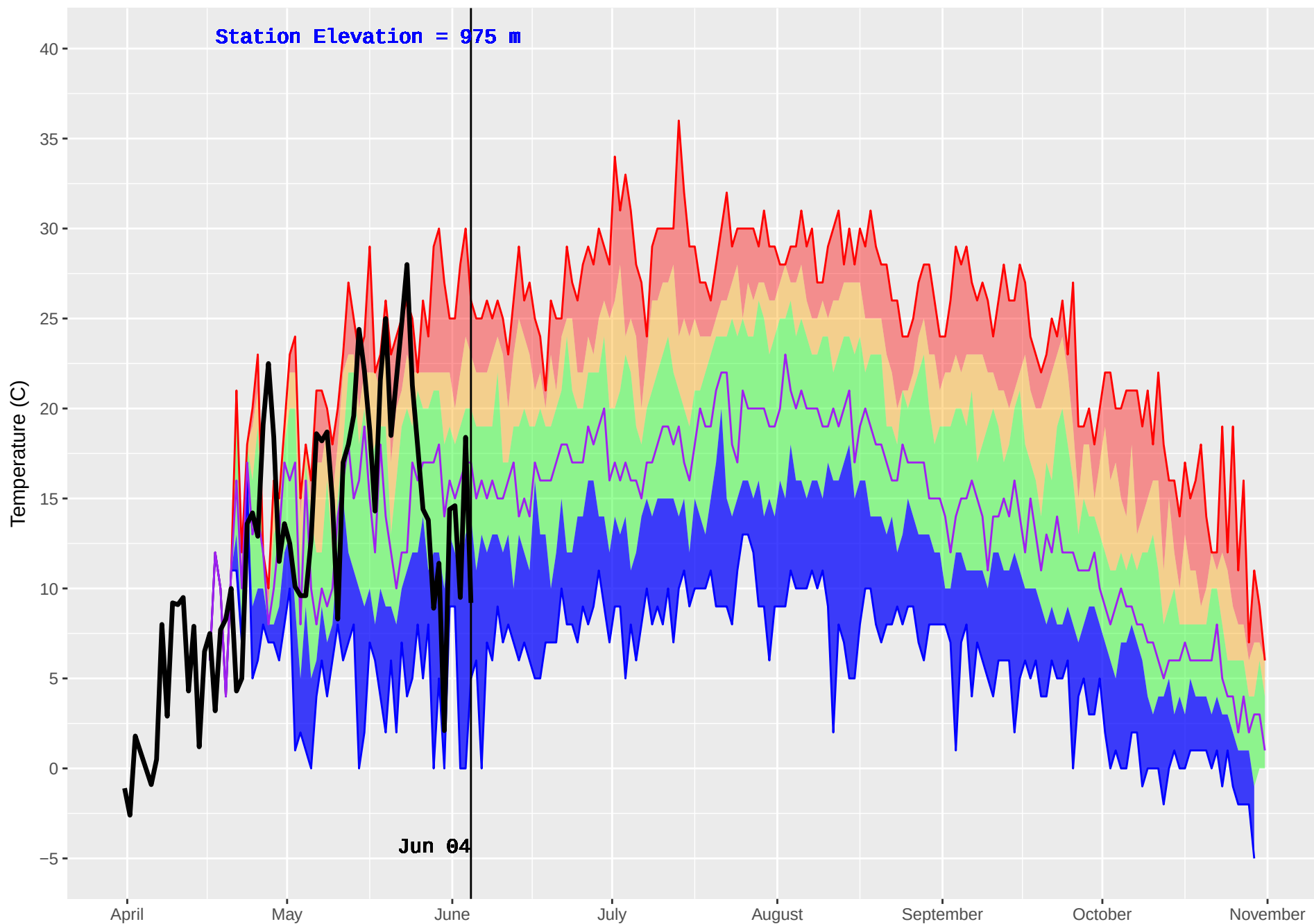
MCGREGOR 2 (192) : Historical (1986–2016) and Current (2018) Noon Temperature
