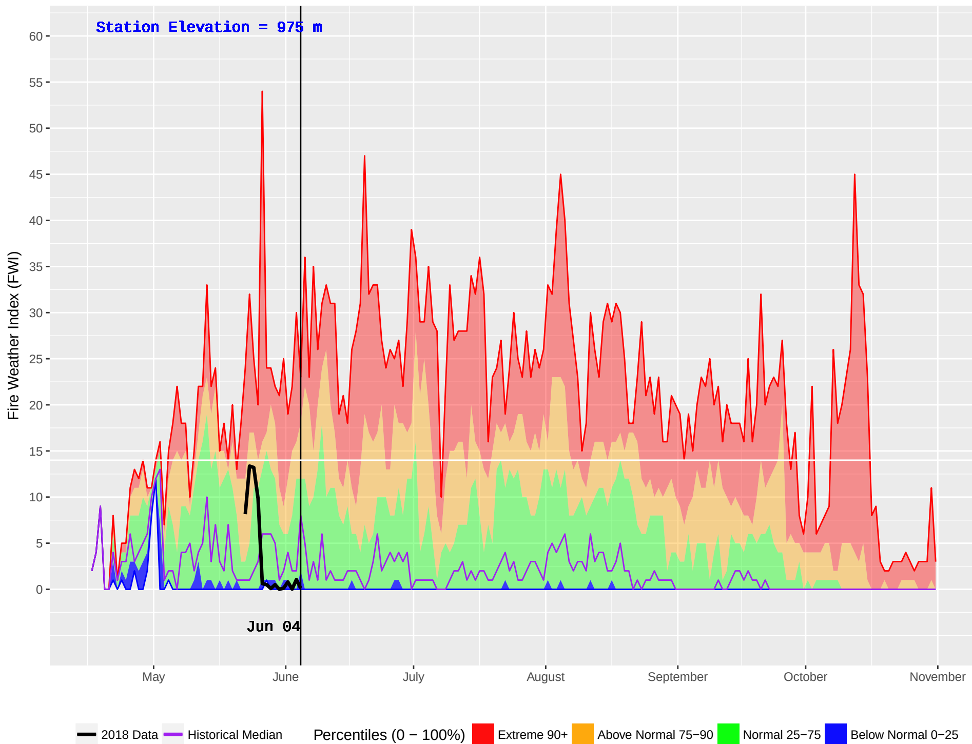
MCGREGOR 2 (192) : Historical (1986–2016) and Current (2018) Noon Fire Weather Index (FWI)
